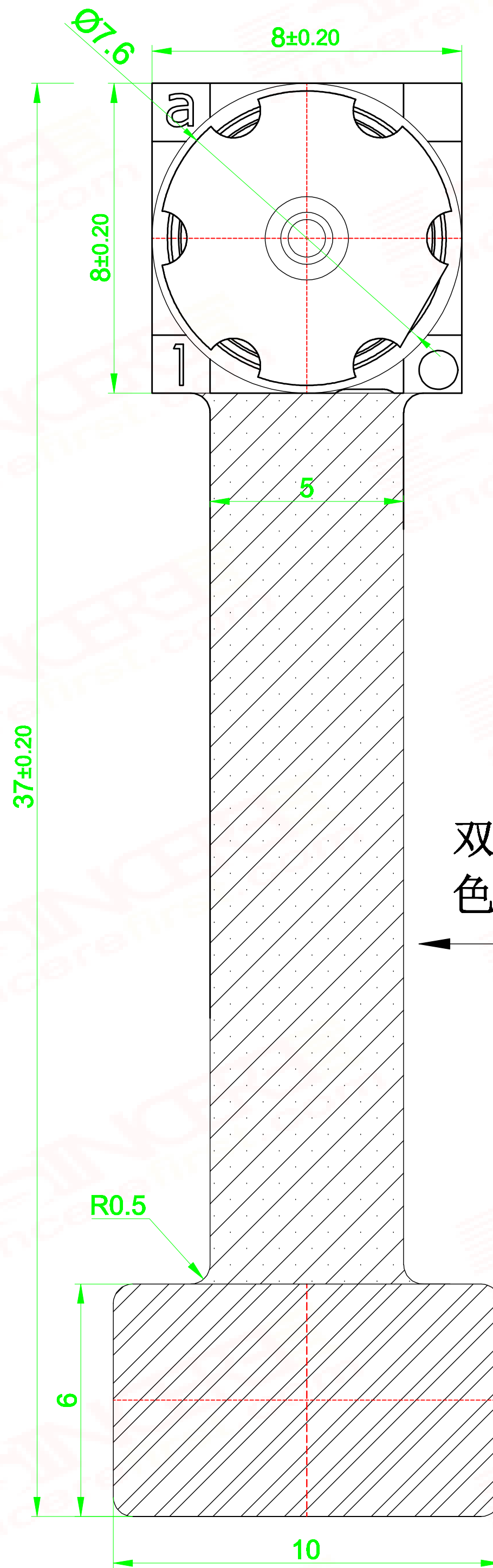
TOP VIEW
