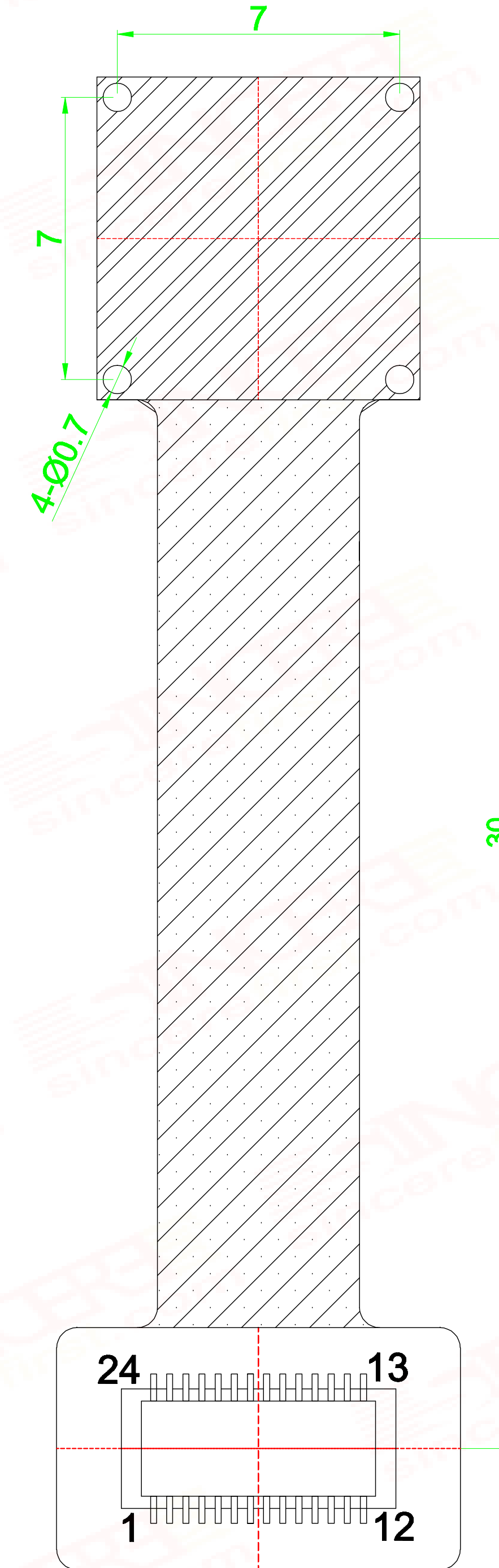
BOTTOM VIEW
