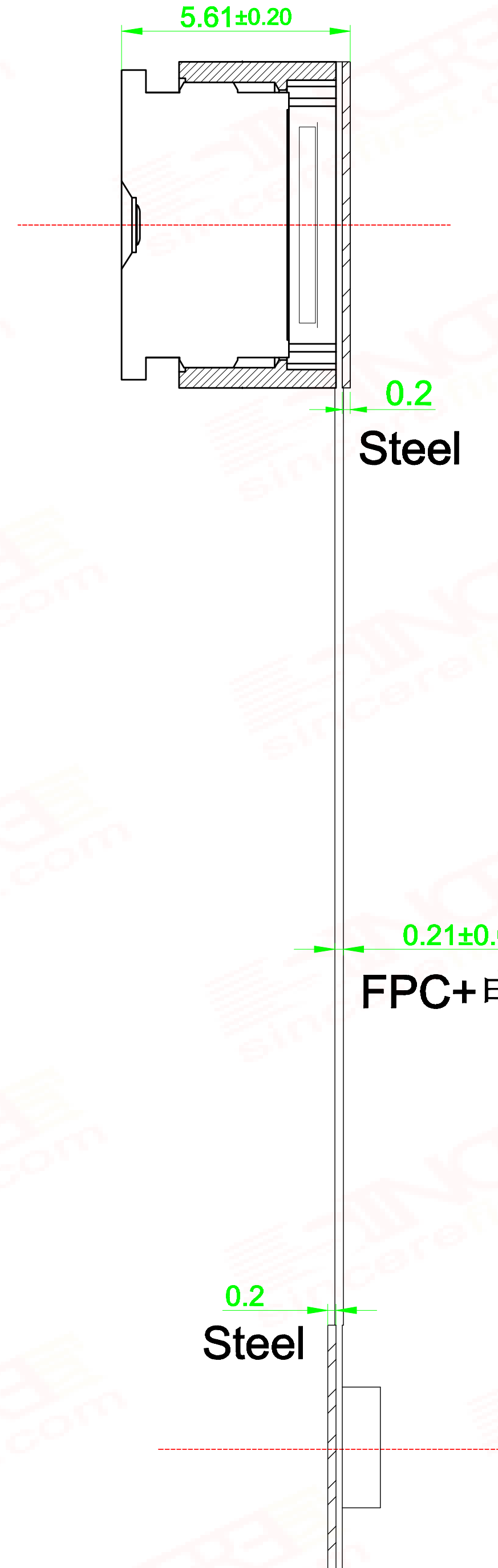
SIDE VIEW
